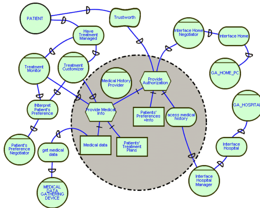
Figure 5. Extended GA PDA Actor Diagram in the Late Requirements
