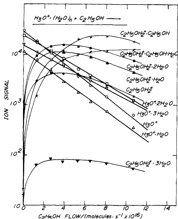
Figure 4. Variation in the ion signals recorded upon the addition of ethanol into a flowing \text{H}_2\text{O}-\text{H}_2 plasma containing hydrated \text{H}_3\text{O}^+ ions. P = 0.316 Torr, L = 84 cm, \bar{v} = 7.7 \times 10^3 cm \text{s}^{-1} , and T = 298 K. The decays provide rate constants of 2.80 , 2.63 , 1.96 , and 1.64 \times 10^{-9} cm ^3 molecule ^{-1} s ^{-1} for the reactions of \text{H}_3\text{O}^+ , \text{H}_3\text{O}^+\cdot\text{H}_2\text{O} , \text{H}_3\text{O}^+\cdot(\text{H}_2\text{O})_2 , \text{H}_3\text{O}^+\cdot(\text{H}_2\text{O})_3 , respectively.
