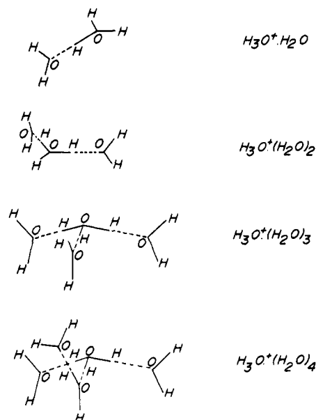
Figure 8. Structures of hydrated \text{H}_3\text{O}^+ ions adopted from the results of ab initio molecular orbital calculations reported by Newton and Ehrenson 26 and Newton. 27
