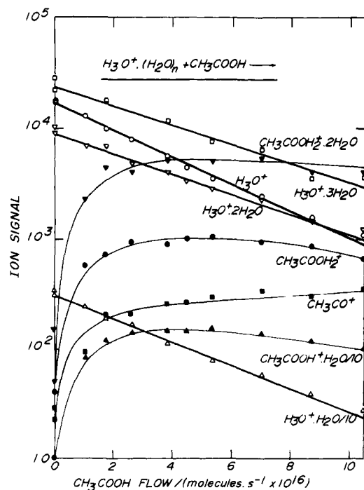
Figure 5. Variation in the ion signals recorded upon the addition of acetic acid into a flowing \text{H}_2\text{O}-\text{He} plasma containing hydrated \text{H}_3\text{O}^+ ions. P = 0.364 Torr, L = 59 cm, \bar{v} = 7.7 \times 10^3 cm \text{s}^{-1} , and T = 298 K. The decays provide rate constants of 3.35 , 2.92 , 2.45 , and 2.29 \times 10^{-9} cm ^3 molecule ^{-1} s ^{-1} for the reactions of \text{H}_3\text{O}^+ , \text{H}_3\text{O}^+\cdot\text{H}_2\text{O} , \text{H}_3\text{O}^+\cdot(\text{H}_2\text{O})_2 , and \text{H}_3\text{O}^+\cdot(\text{H}_2\text{O})_3 , respectively.
