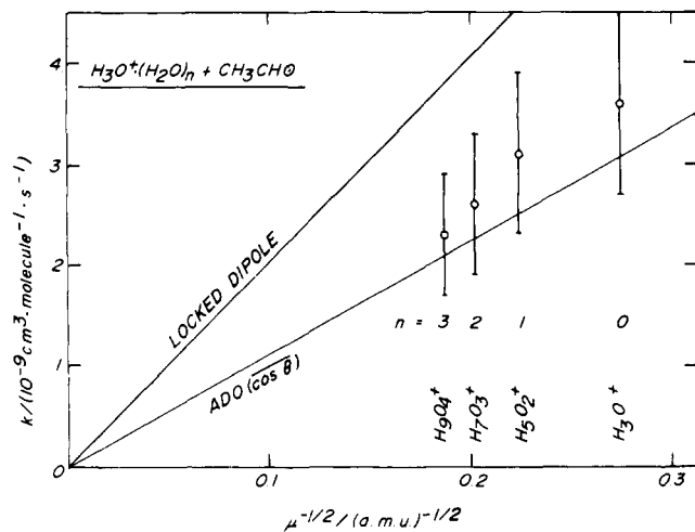
Figure 7. A comparison of the measured rate constants with rate constants predicted by collision theories for the reactions of hydrated \text{H}_3\text{O}^+ ions with acetaldehyde ( \alpha = 4.40 \text{ \AA}^3 , \mu_D = 2.69 \text{ D} ) at 298 \pm 2 \text{ K} . The solid bars represent the estimated accuracy of the measurements.
