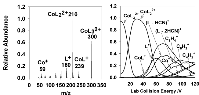
Figure 2. CID spectrum of m/z = 300 ( [\text{CoL}_3]^{2+} ) at 25 V and CID profiles monitored for the dissociation of [\text{CoL}_3]^{2+} up to 120 V. L = 1,10-phenanthroline.
