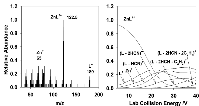
Figure 4. CID spectrum of m/z = 122.5 ( [\text{ZnL}]^{2+} ) at 20 V and CID profiles monitored for the dissociation up to 40 V. L = 1,10-phenanthroline. Ion collection appears to discriminate against the \text{Zn}^+ ion by a factor of about 2.4, presumably due to its relative velocity.
